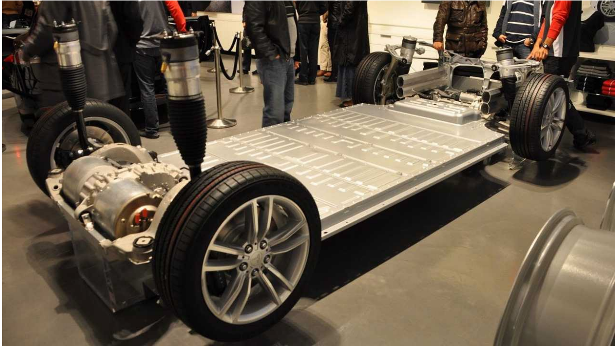
Figure 24 One example of the BEV skateboard design. Source: https://insideevs.com/news/450534/tesla-leaves-skateboard-design-new-structural-battery-packs/
